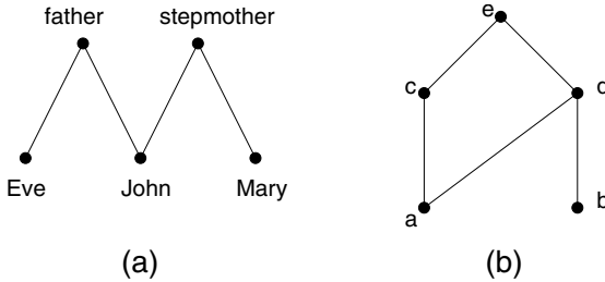
Fig. 2. (a) patchwork families, (b) \mathbf{a} is a candidate for being one’s own cousin
