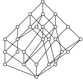
Fig. 1. Data table with fuzzy attributes and fuzzy concept lattice
