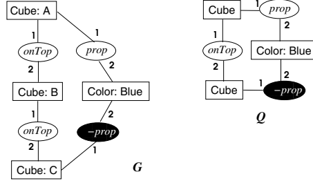
Fig. 1. Atomic negation
