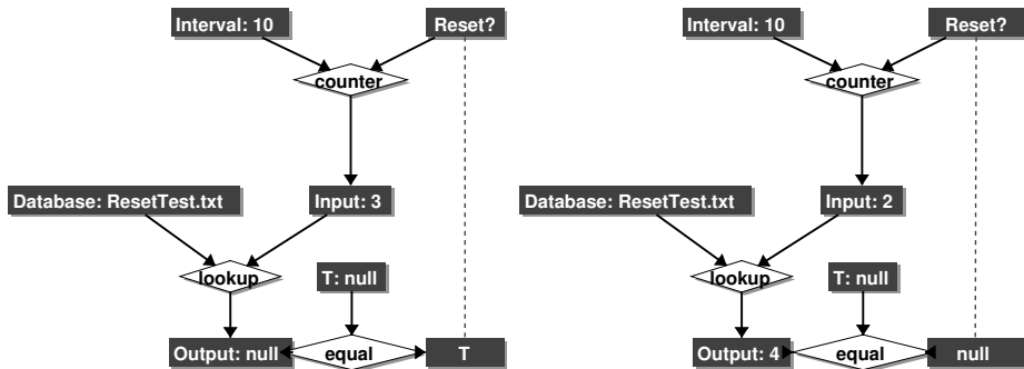
Fig. 4. Two examples using the <counter> actor
