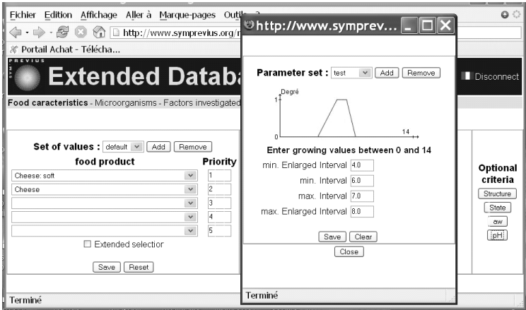
Fig. 4. The GUI permits to define a trapezoidal fuzzy set which represents the end-user’s preferences for the numerical attribute pH
