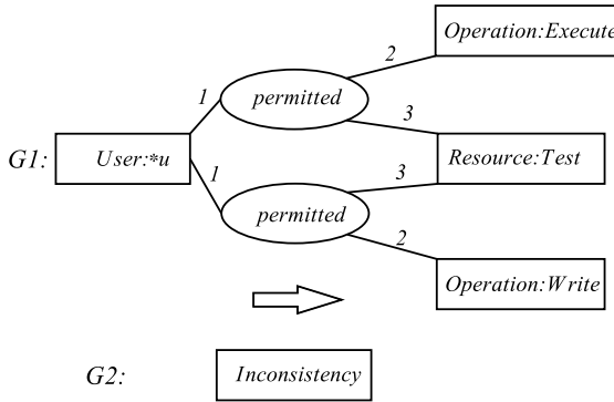
Fig. 7. No user can be permitted both Execute and Write operations on Test
