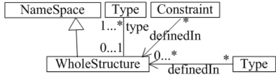
Fig. 3. The metamodel of whole structure
