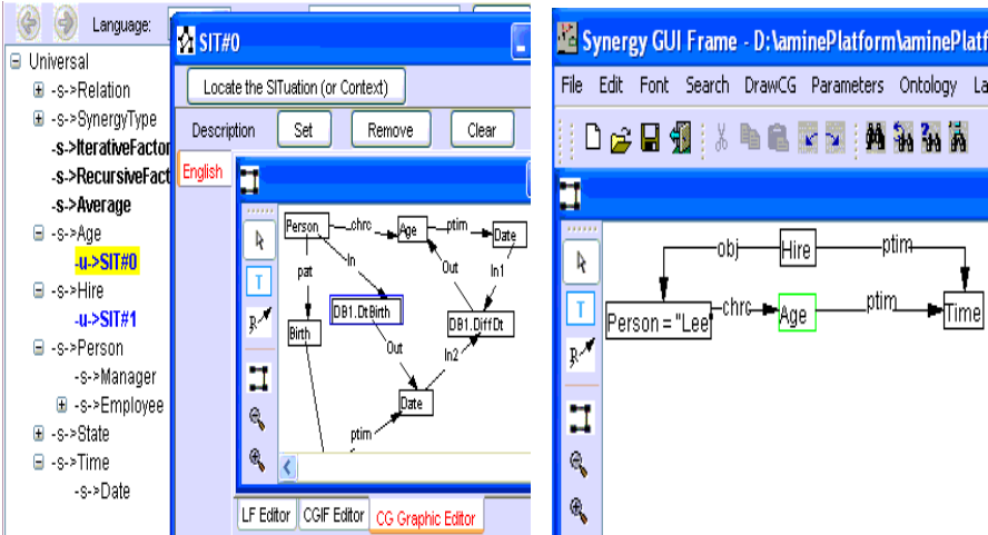
(a) Snapshot of the ontology b) The request: initial state of the WG
